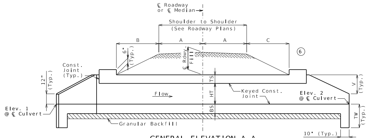
GENERAL ELEVATION A-A
