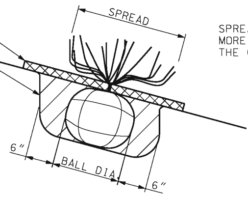
EVERGREEN SHRUB SLOPE PLANTING
