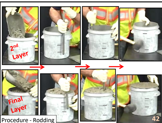
Procedure - Rodding 42
