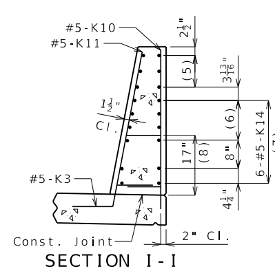
ALTERNATE DETAILS FOR SKEWED BRIDGES REQUIRING K3 BARS
