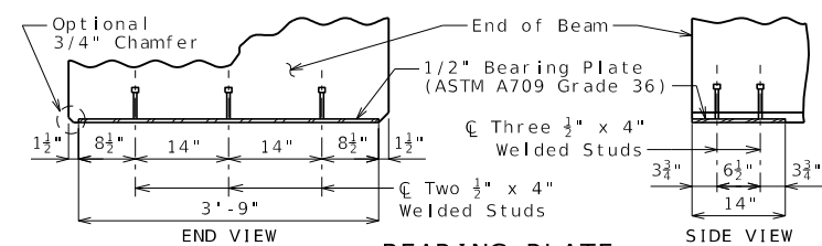
BEARING PLATE
