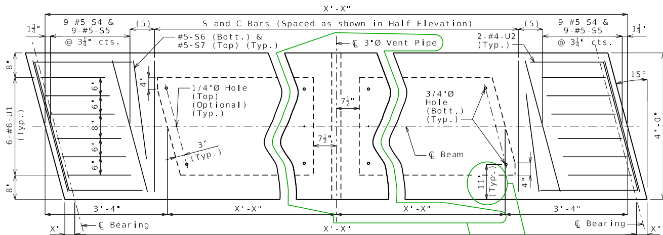
PART PLAN
