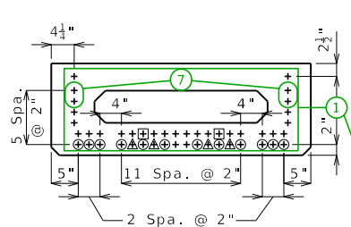
STRAND ARRANGEMENT
