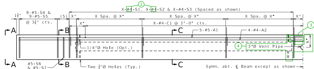
HALF ELEVATION
