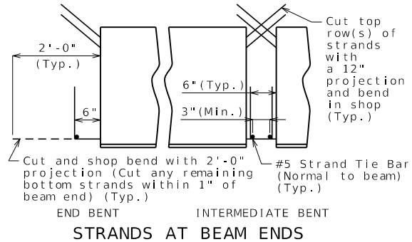
STRANDS AT BEAM ENDS
