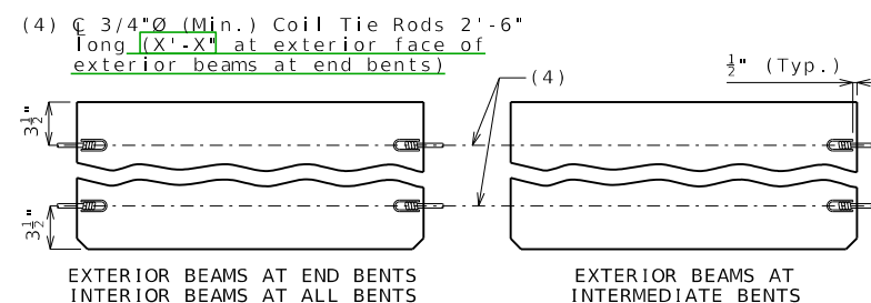
COIL TIES
