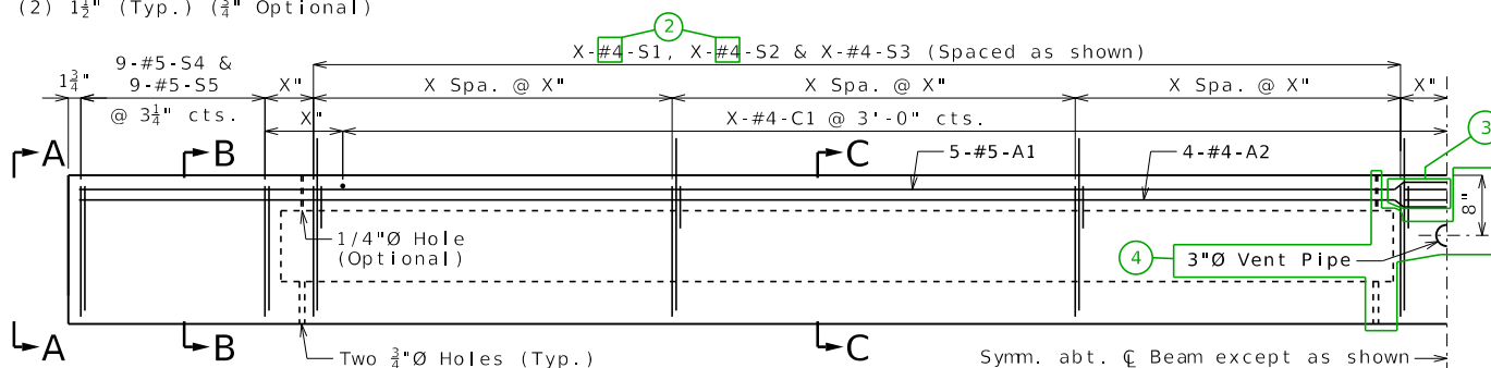
HALF ELEVATION
