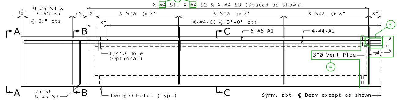
HALF ELEVATION
