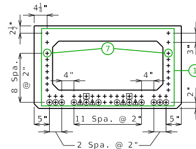
STRAND ARRANGEMENT
