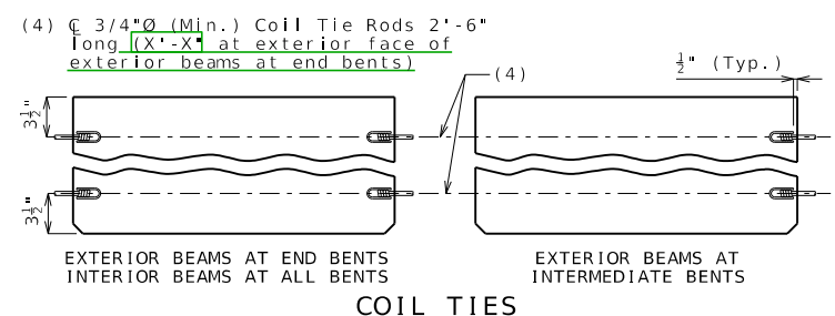
COIL TIES
