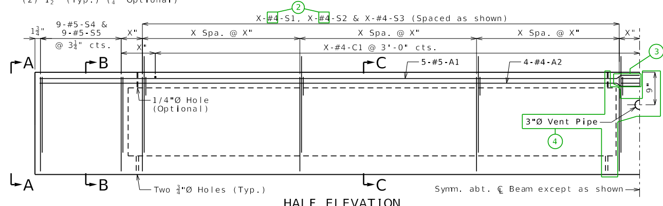
HALF ELEVATION
